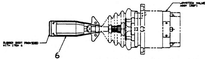
HANDLE INSTL W/O HOIST ROTATION INDICATOR
