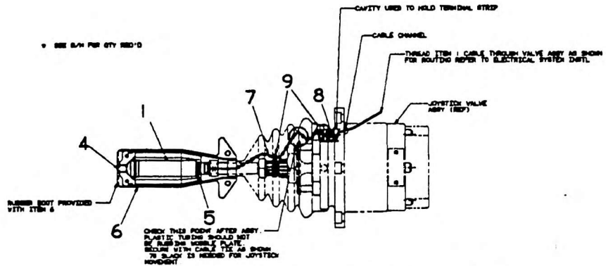
HANDLE INSTL WITH HOIST ROTATION INDICATOR
